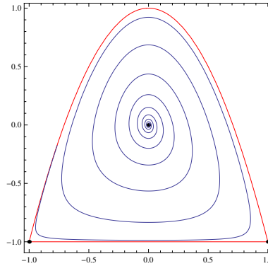
Figure 7.9. Phase portrait of an example where \omega_\sigma(x) consists of fixed points and orbits connecting them
