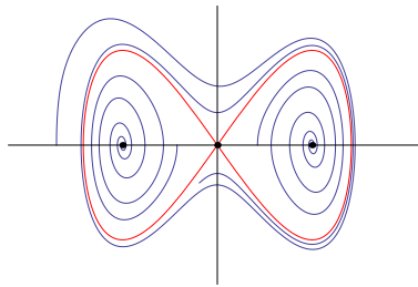
Figure 7.10. Phase portrait of an example where \omega_\sigma(x) consists of leaves
