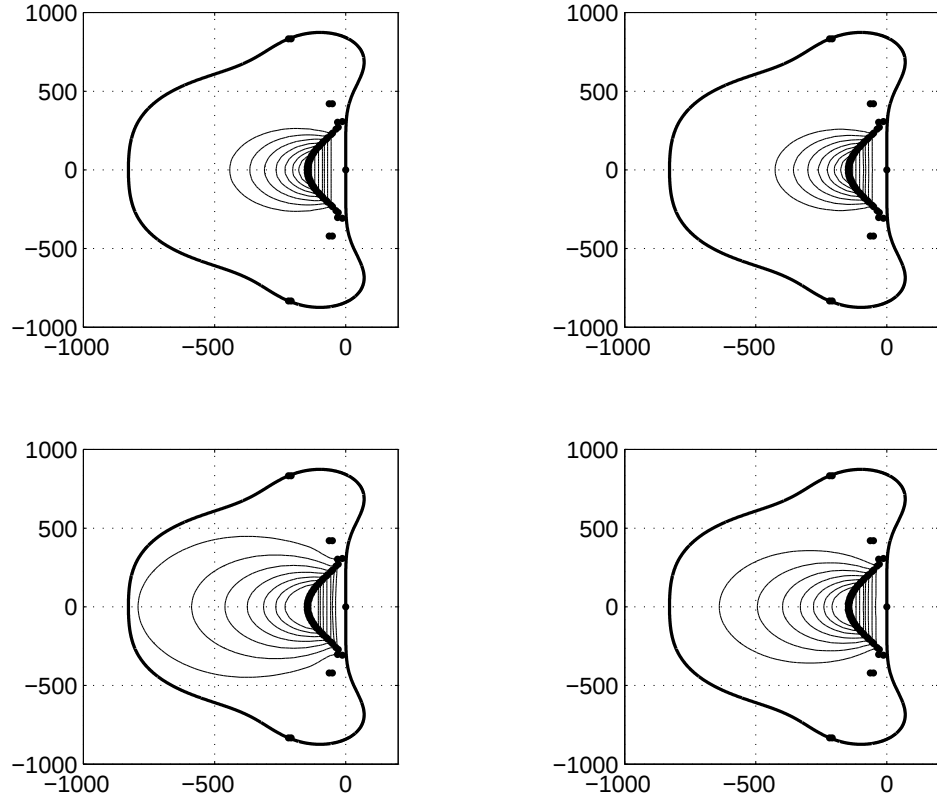
Figure 2: Region of absolute stability of fourth-order Runge-Kutta method scaled by 1/\Delta t_{\max} and spectra and \epsilon -pseudospectra of system matrices A_1 (top left) A_2 (top right), A_3 (bottom left), and A_4 (bottom right), for \epsilon = 10^{-9}, 10^{-8}, \dots, 10^{-3} (from inner to outer), n = 31 , c = 5 , and \Delta t_{\max} = 0.01680
