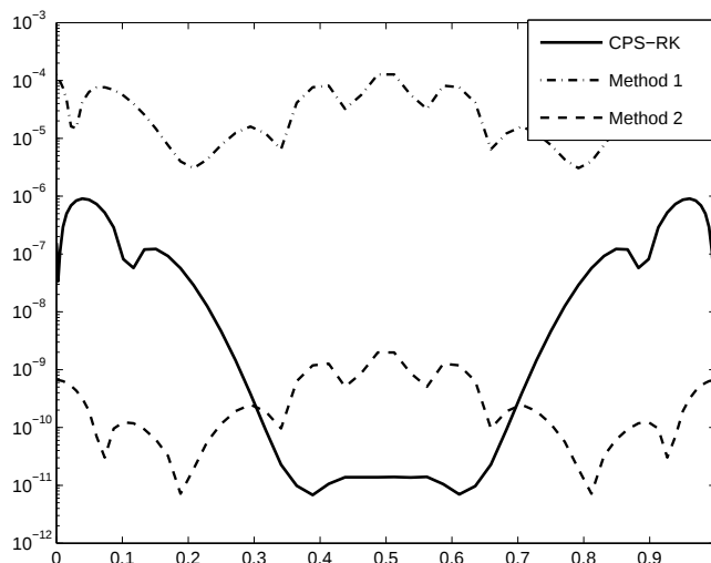
Figure 4: Error in absolute value of approximate solutions at time level t = 0.12
