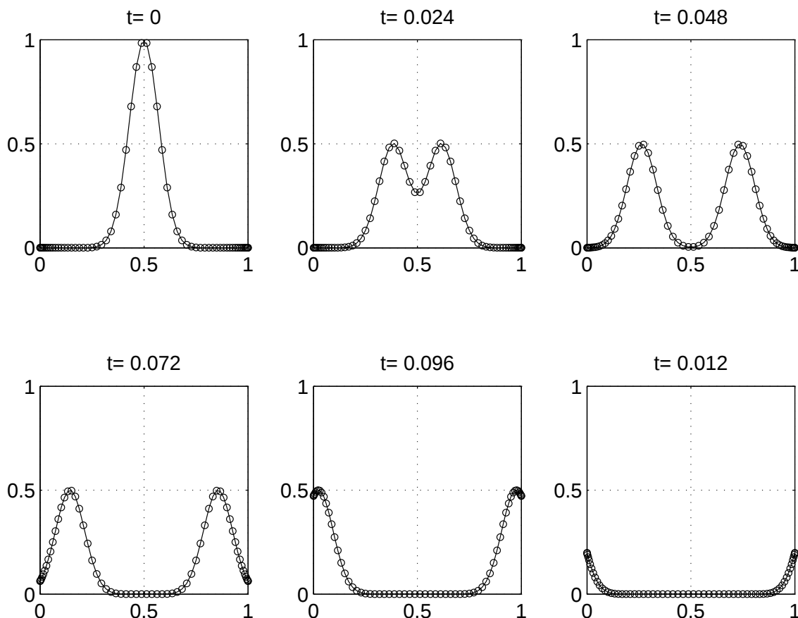
Figure 3: Exact and CPS-RK-based approximate solution for 1D wave equation
