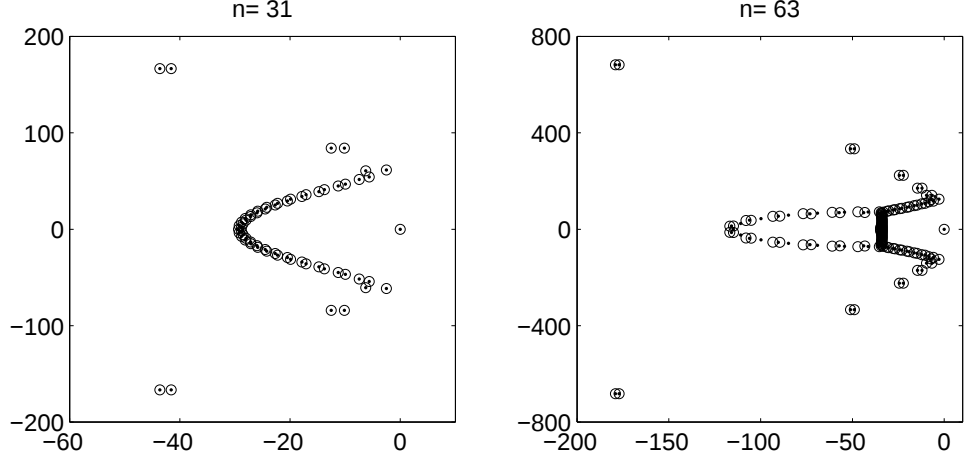
Figure 1: Eigenvalues of system matrices A_1 (circles) and A_2 (dots).
