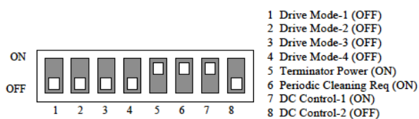
DIP Switch Positions
