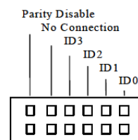
Figure 3-3: Jumper positions
