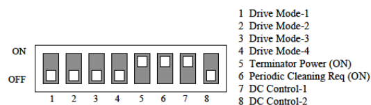
DIP Switch positions
